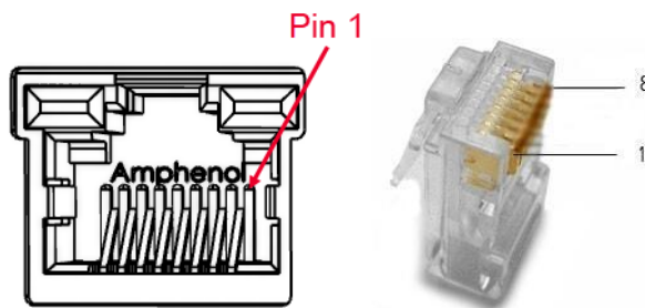
Figure 3. ZED CAN interface (C3, C4) and connector
