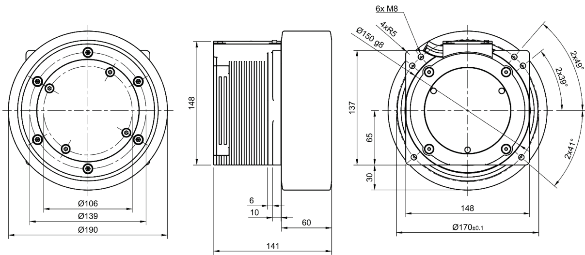
Figure 9-1. MOT-HM 0303 Dimensions
