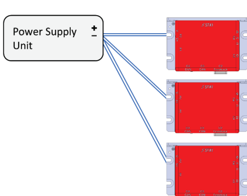
Figure 1. Star Connection
