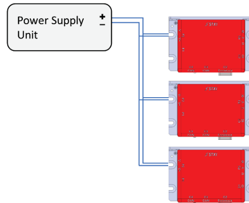
Figure 2. Bus Connection
