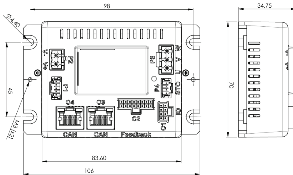
Figure 5-1 SD01-015 dimensions
