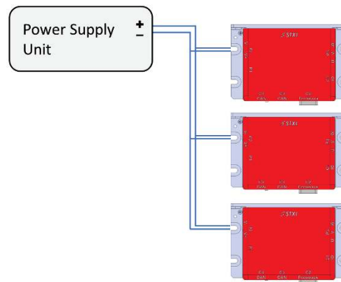
Figure 2. Bus Connection
