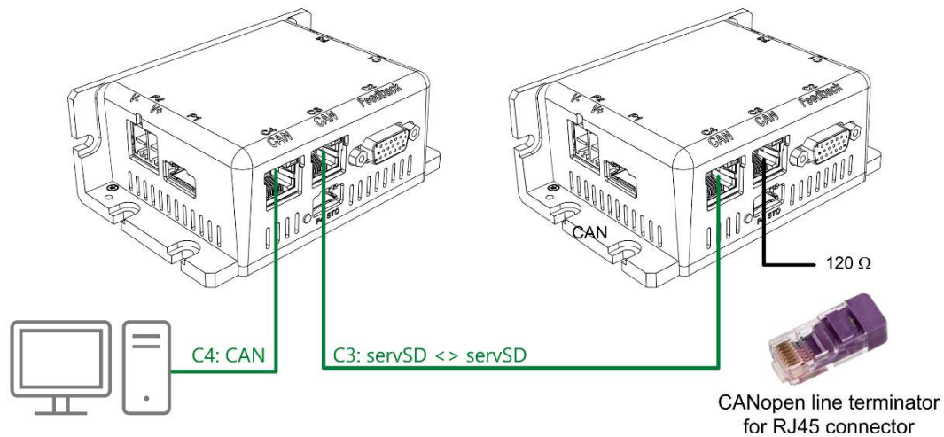
Figure 6. servSD CAN Network Configuration
