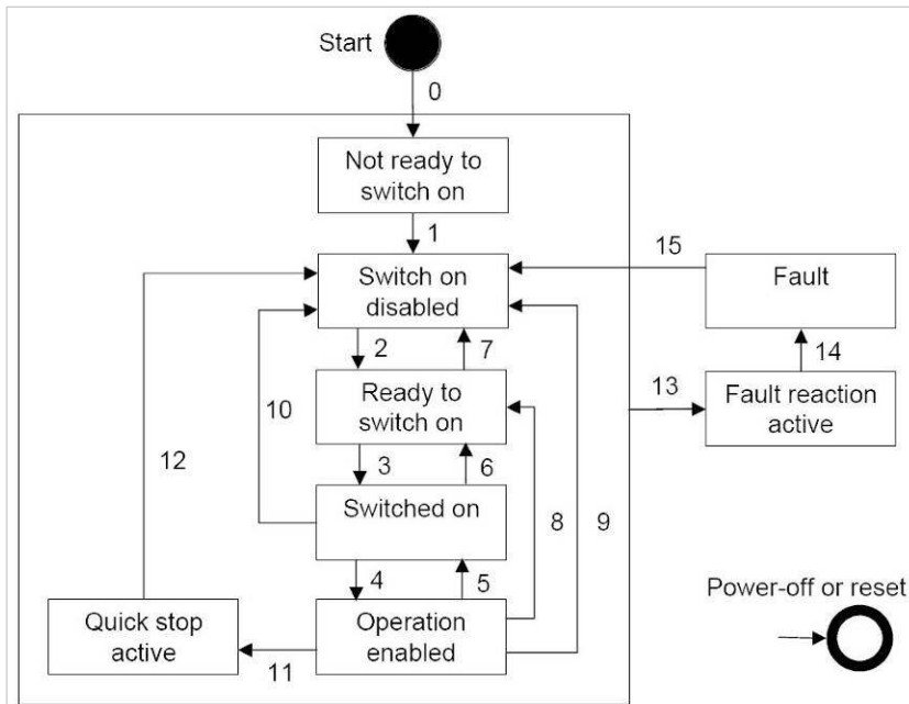
Figure 9. Power Drive System State Diagram
