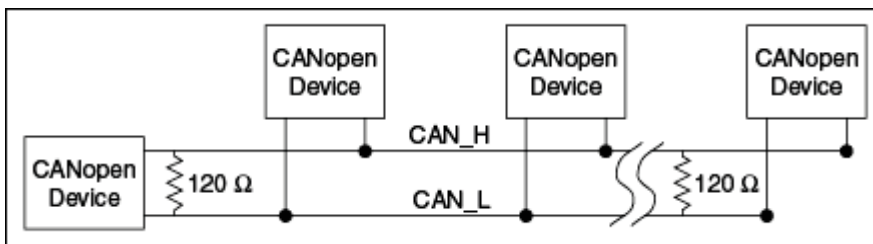
Figure 5. Placement of terminator resistors
