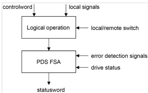
Figure 8. Remote and Local Control
