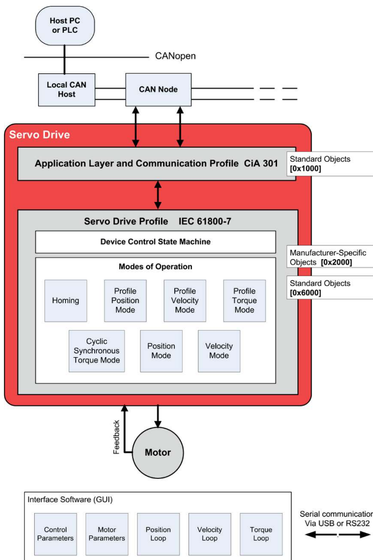
Figure 7. Communication Architecture
